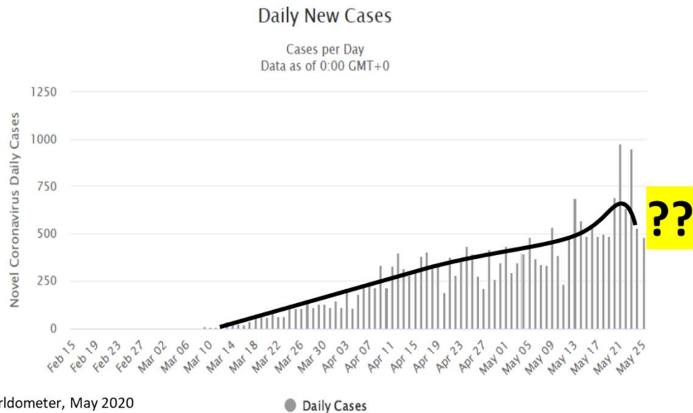
Daily New Cases in Indonesia
